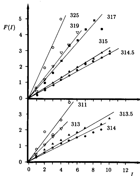
FIGURE 4 The function F(I) in Eq. 5 shown at different temperatures above and below the transition temperature for the case of a seven-site protein with a hydrophobic length of d_p = 18 \text{ \AA} (cf. Fig. 5). The different data sets are labeled by the value of the temperature (in K).
